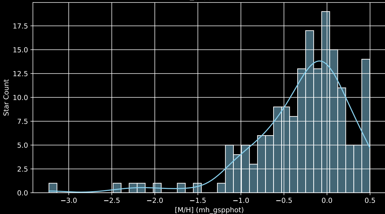
APOGEE DR17 Field: [000-02 [M/H] (mh_gspphot) (n= 175)
