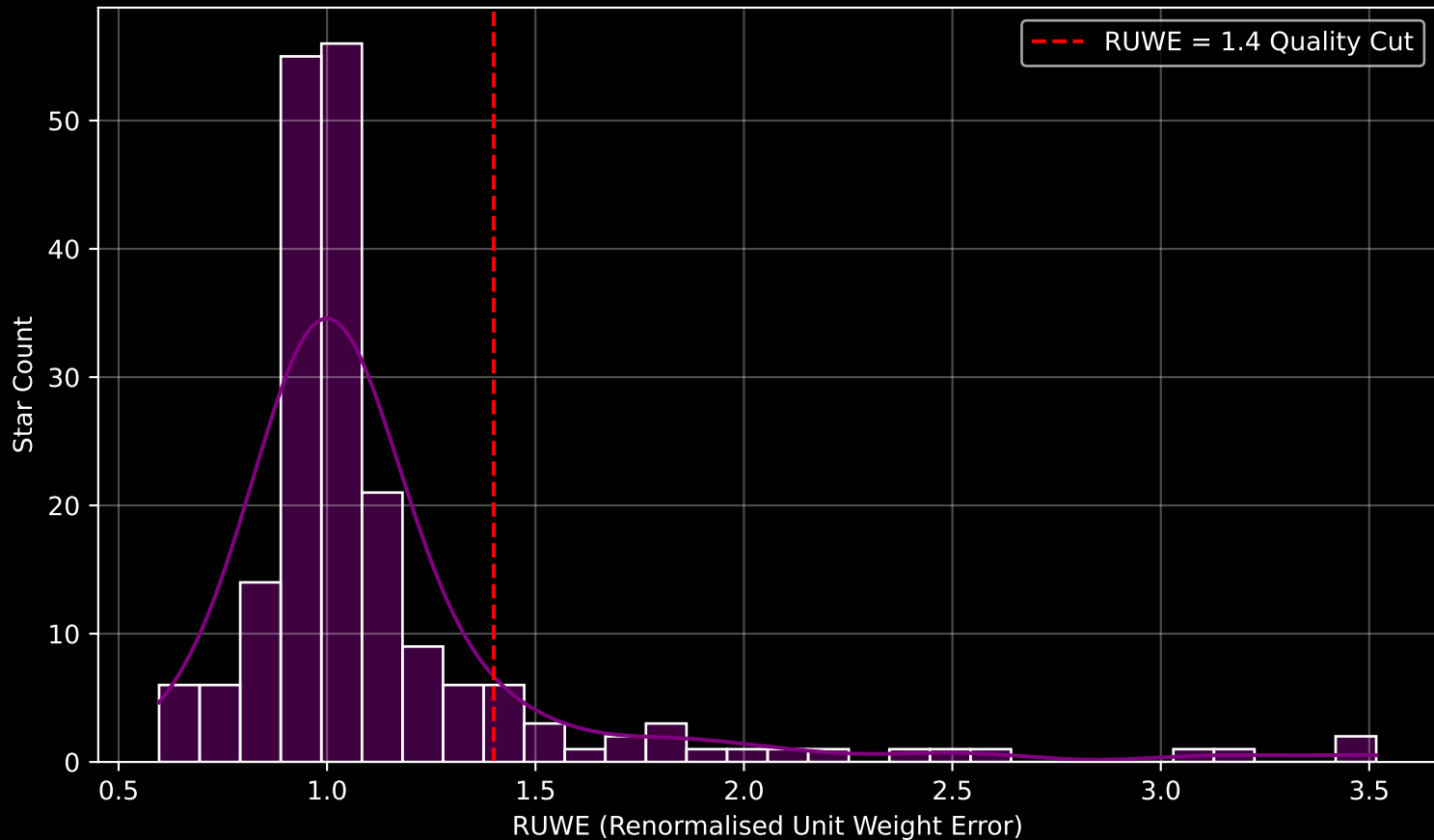
GAPOGEE DR17 Field [000-02] RUWE Distribution (n= 199)
