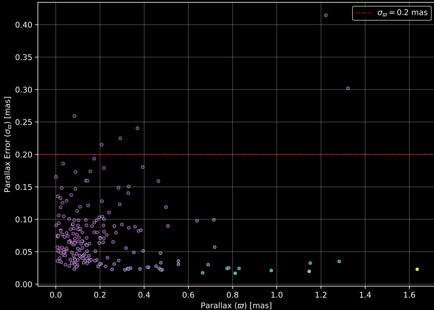
APOGEE DR17 Field: [000-02] Parallax Quality (n = 200)
