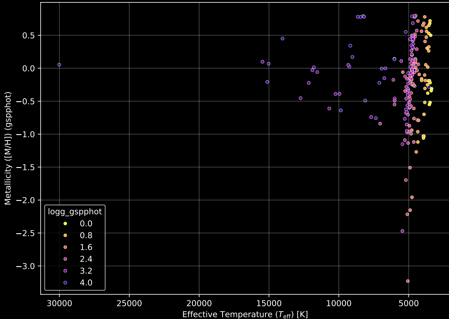
APOGEE DR17 Field: [000-02] Stellar Population Parameters (n= 200)
