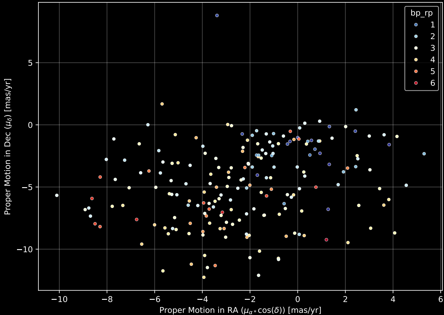
APOGEE DR17 Field: [000-02] Proper Motion Diagram (n= 200)
